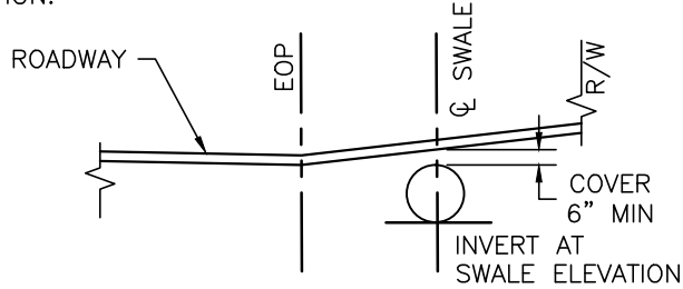
SECTION VIEW DRIVEWAY W/CULVERT
