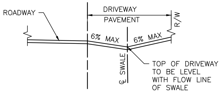
SECTION VIEW DRIVEWAY W/SWALE
