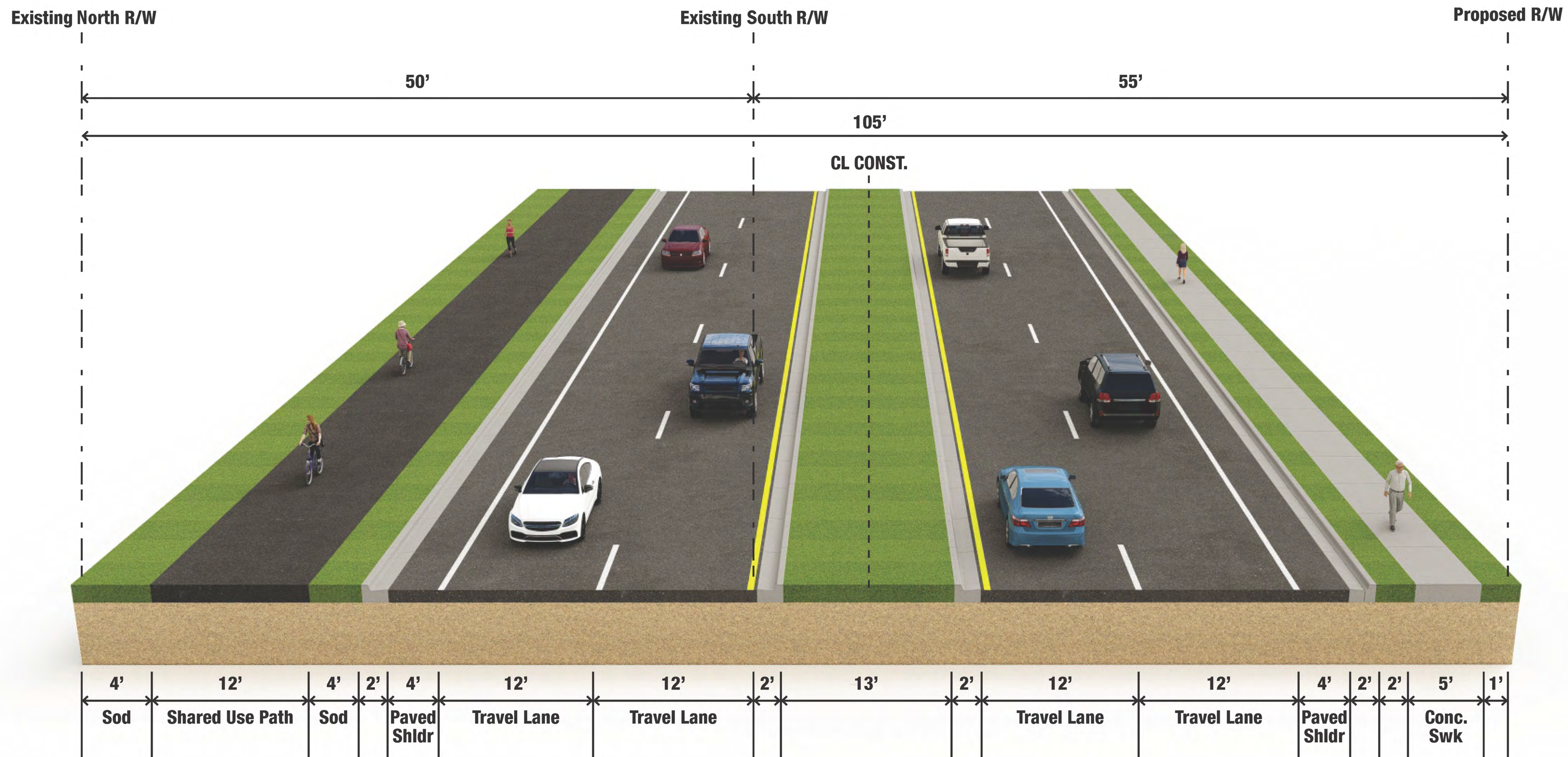
Typical Section 3A From SW 46th Avenue to SW 43rd Court
