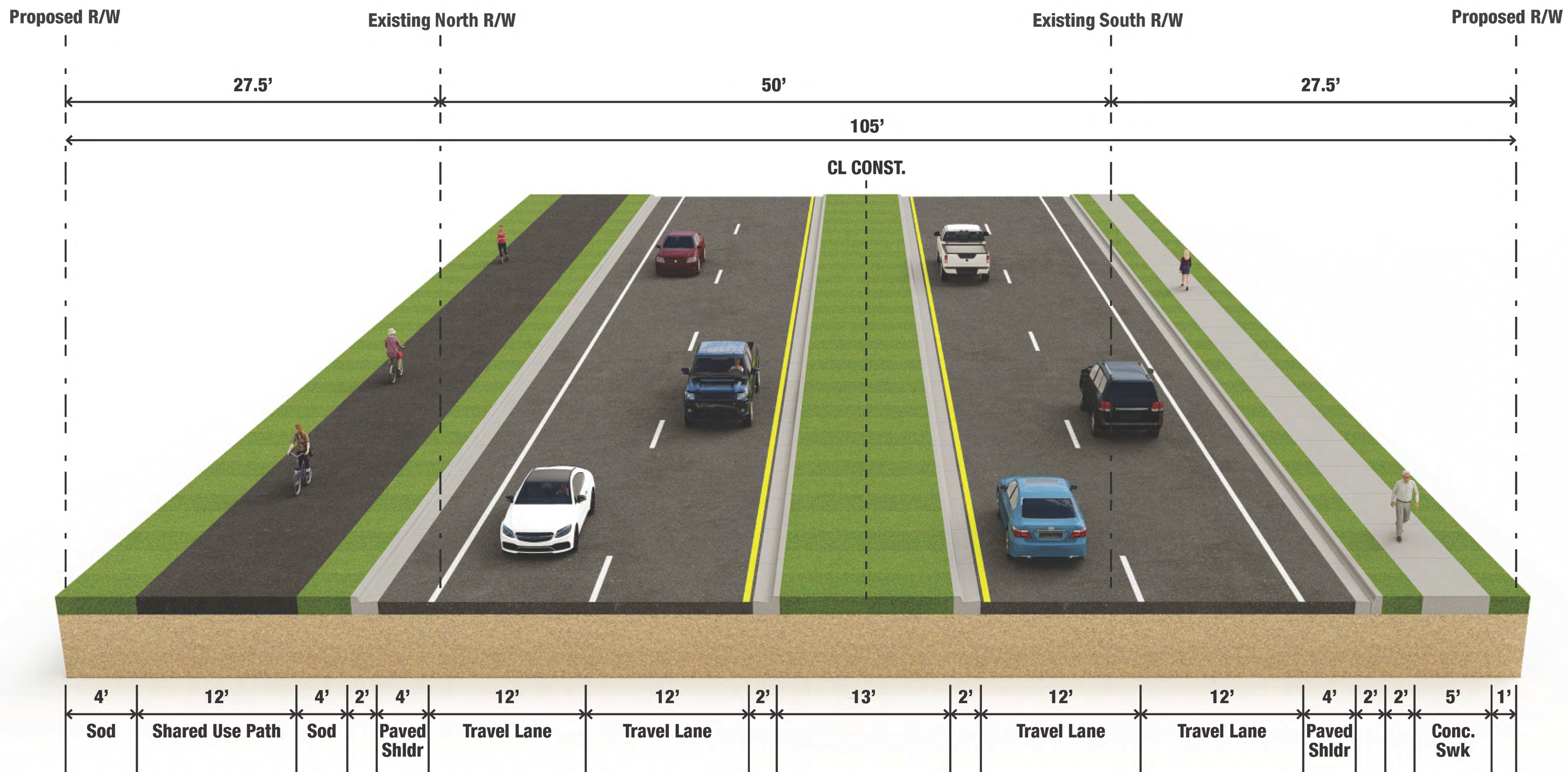
Typical Section 3B From SW 46th Avenue to SW 43rd Court
