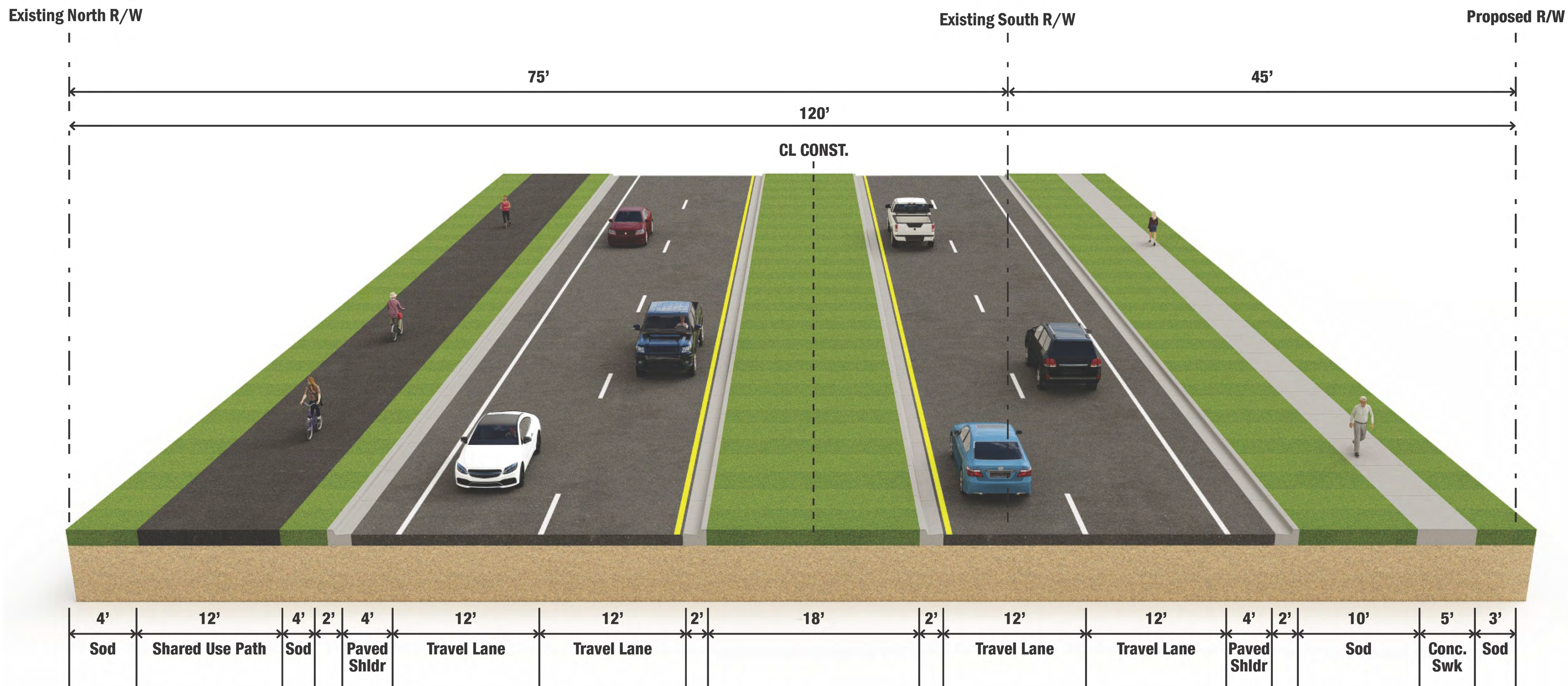
Typical Section 1A From SW 80th Avenue to SW 60th Avenue
