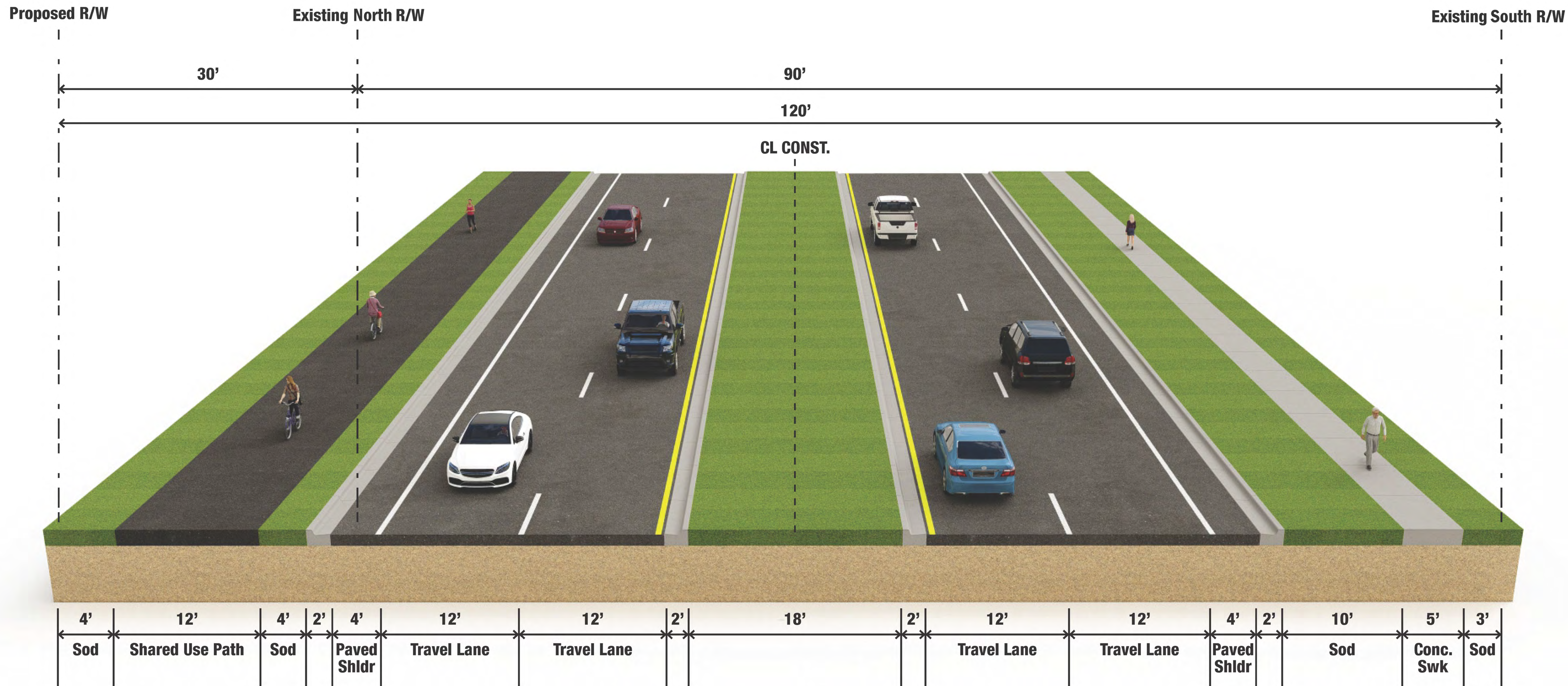
Typical Section 2B From SW 60th Avenue to SW 46th Avenue
