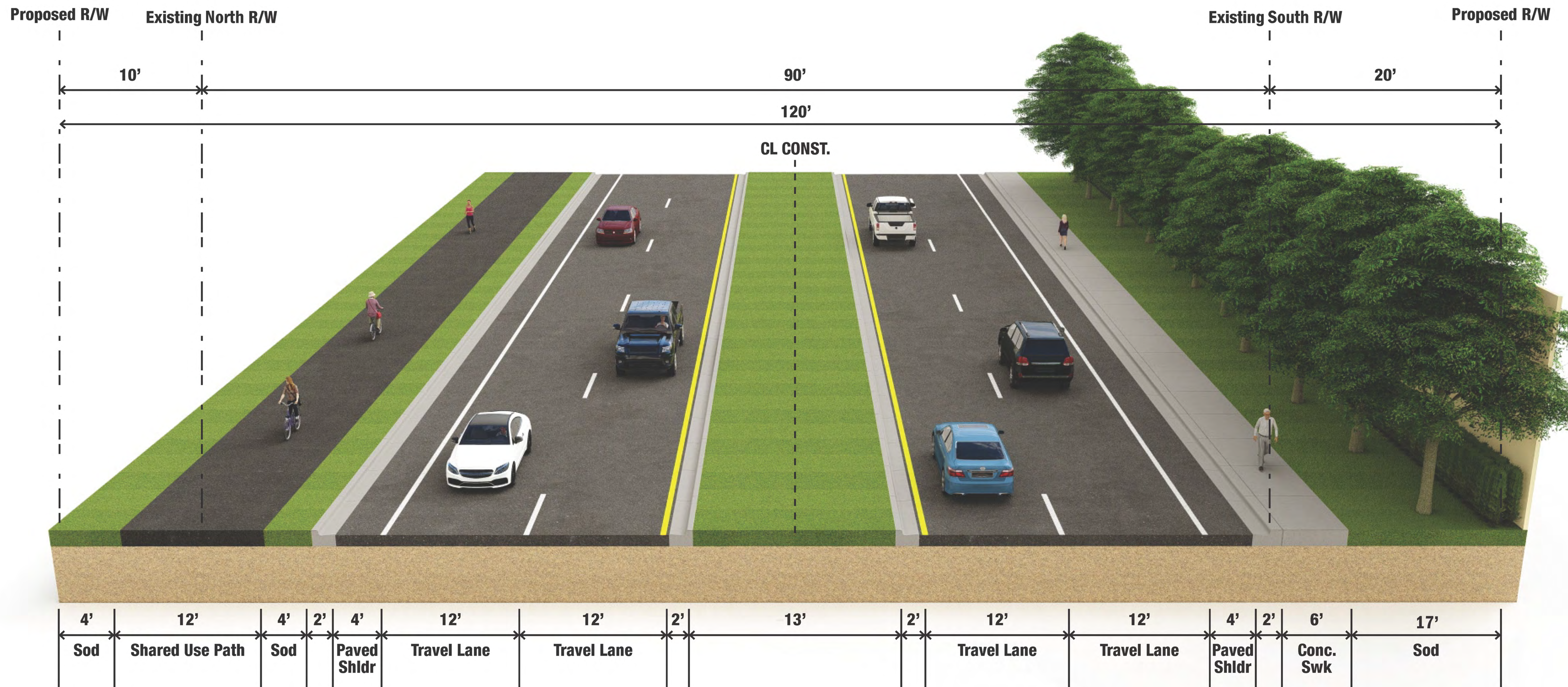
Typical Section 2A From SW 60th Avenue to SW 46th Avenue
