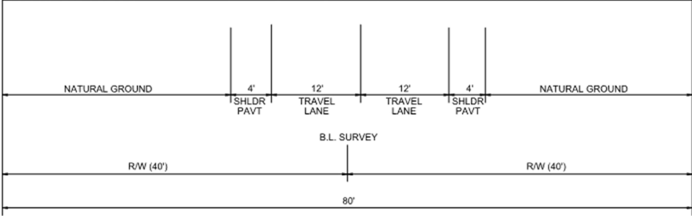
SW 49 th Avenue – Existing Typical Section
